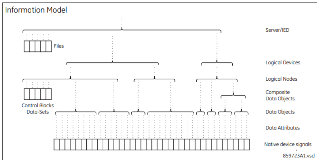
Figure 2: ACSI block
